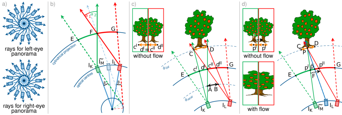
Figure 2.6.: (a) Illustration of rays required for creating a stereoscopic panorama and (b) deviation angles \alpha . (c) Duplication and truncation artefacts caused by the aliasing. (d) Flow-based upsampling to synthesize required rays. Adapted from [RPZSH13]
