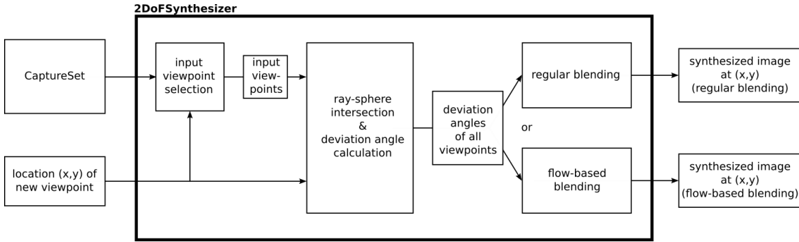
Figure 3.8.: System diagram of the 2DoFSynthesizer
