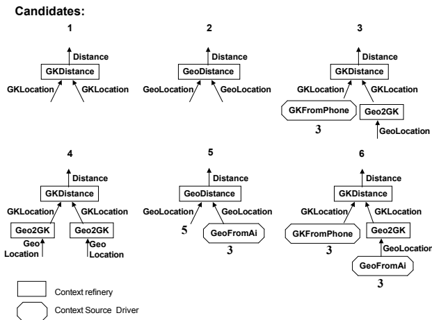
Figure 7 Finding a Tree of Refinement Components in CAIMS
