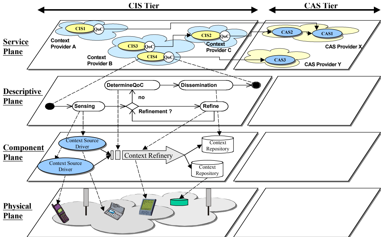
Figure 3 A Framework for Context Provisioning
